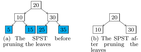
Figure 3: The SPST with size n = 7 being pruned.
