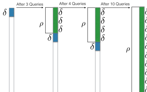
Figure 1: Progressive indexing.
